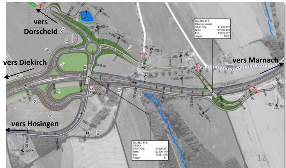
ZOOM 3 Carrefour dénivelé Hosingen-Nord + raccord Lehmkaul – Dorscheid
